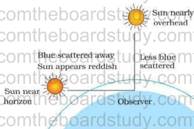
Reddening of the Sun at sunrise and sunset
