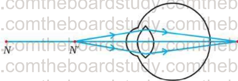
(a) Hypermetropic Eye
