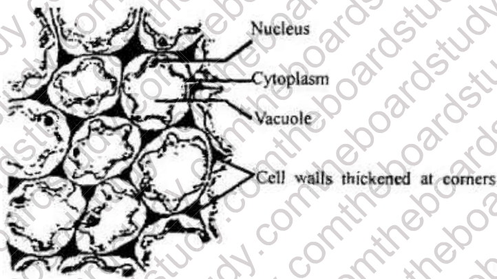
Collenchyma
