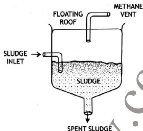
Anaerobic sludge digester.
